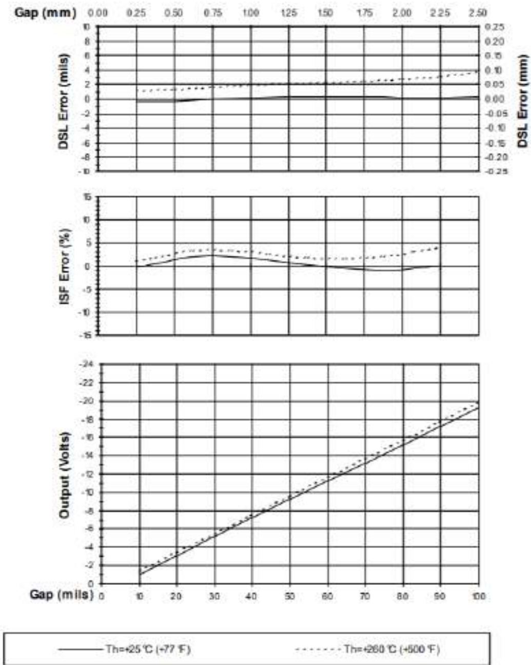
Figure 9: Typical 3300 XL Extended Temperature Range Probe and 8m Extended Temperature Range Extension Cable at T_h (Proximitor Sensor and Probe Tip with 1-foot Cable are at +25\text{ }^{\circ}\text{C} )
