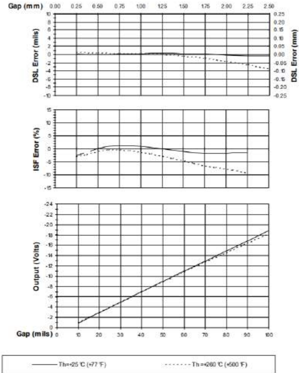
Figure 8: Typical 3300 XL Extended Temperature Range Probe and 4m Extended Temperature Range Extension Cable at T_h (Proximitor Sensor and Probe Tip with 1-foot Cable are at +25\text{ }^{\circ}\text{C} )
