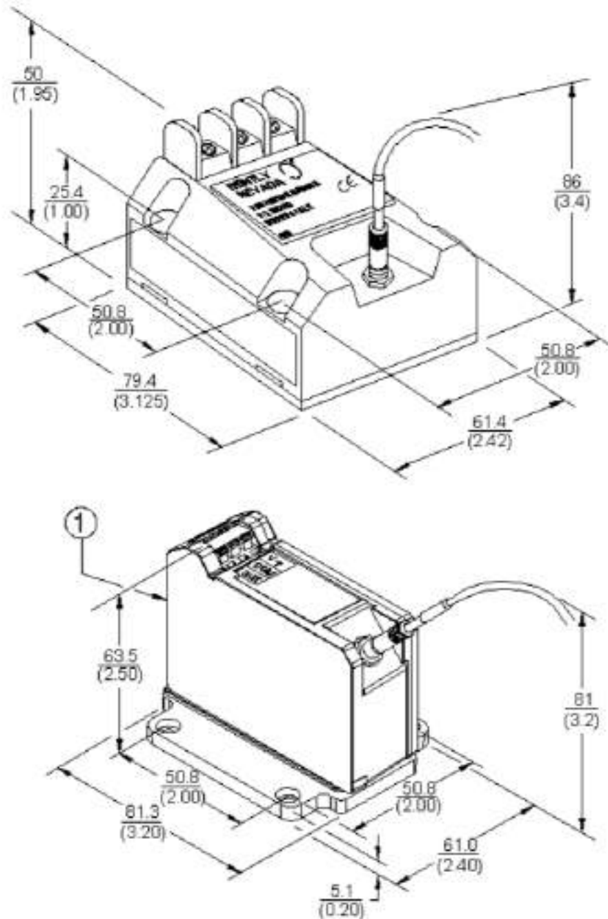
Figure 21: Physical Mounting Characteristics Showing Interchangeability of 3300 and 3300 XL Proximity Sensors when 4-hole Mounting Option Is Used 8
